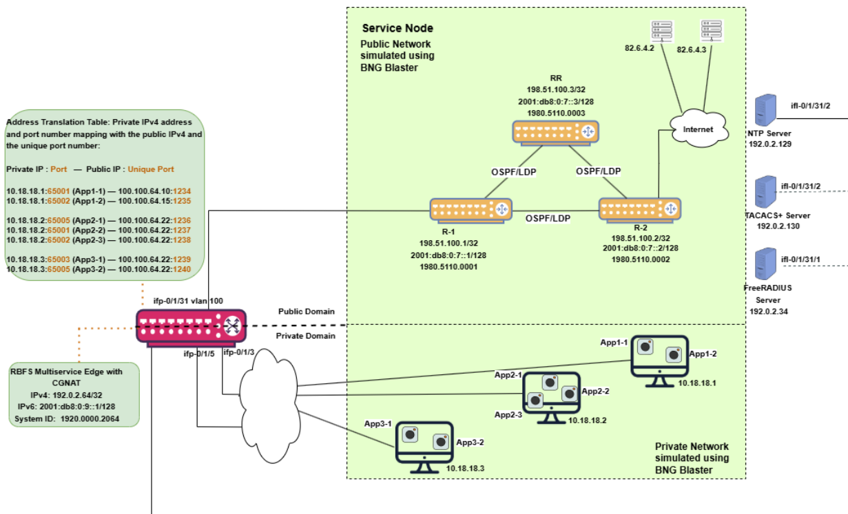
Figure 11. RBFS Multiservice Edge with CGNAT Implementation
